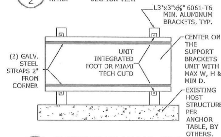
4 ALUMINUM WALL STAND N.T.S. PLAN VIEW
