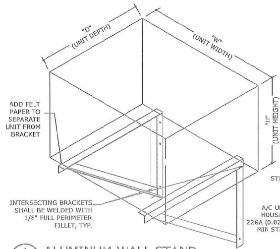
1 ALUMINUM WALL STAND N.T.S. ISOMETRIC VIEW
