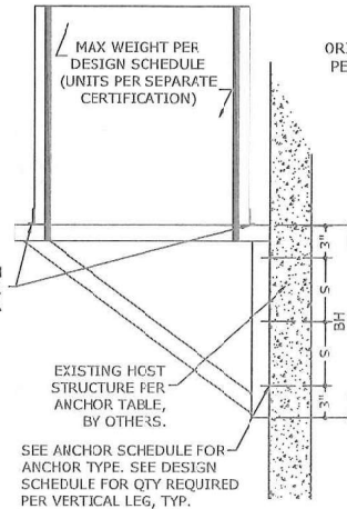
2 ALUMINUM WALL STAND N.T.S. SECTION VIEW
