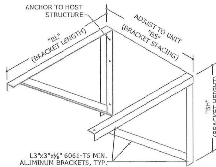
3 ALUMINUM WALL STAND N.T.S. ISOMETRIC VIEW
